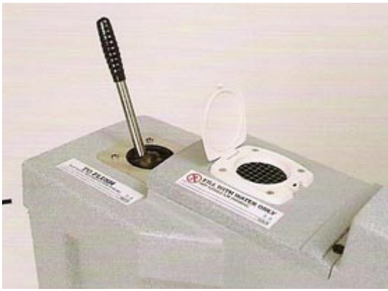
↑ The robust manually operated flushing pump , it is equipped with a vandal-resistant handle and stainless steel mounting plate.
